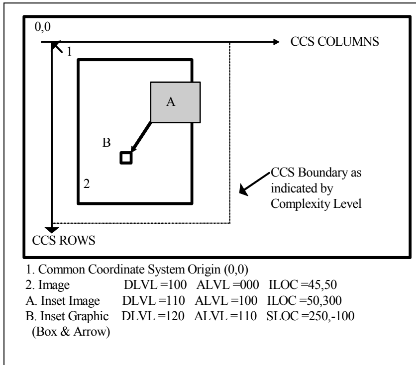
FIGURE 16. Single file, single base image.
